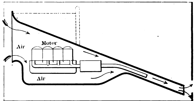
Fig. 59—Energy in the exhaust is used to sweep cooling air over all the motor surfaces
